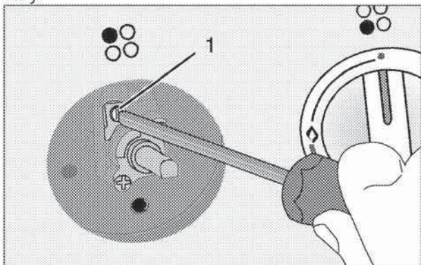
1 Flow rate adjustment screw
