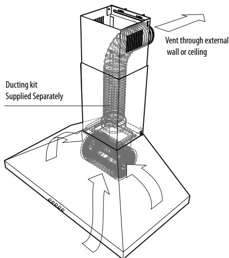
Fig 1. Ducting mode (No charcoal filters required)
