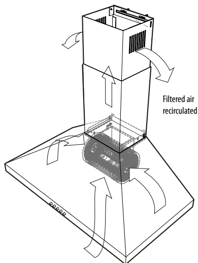
Fig 2. Recirculation mode (Charcoal filters required)
