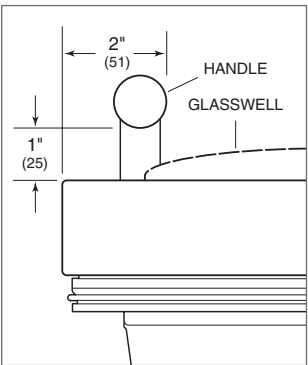
Handle placement.
