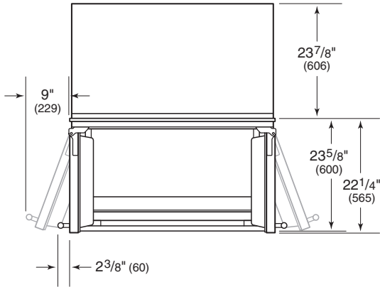
Model BI-42UFD(ID).
